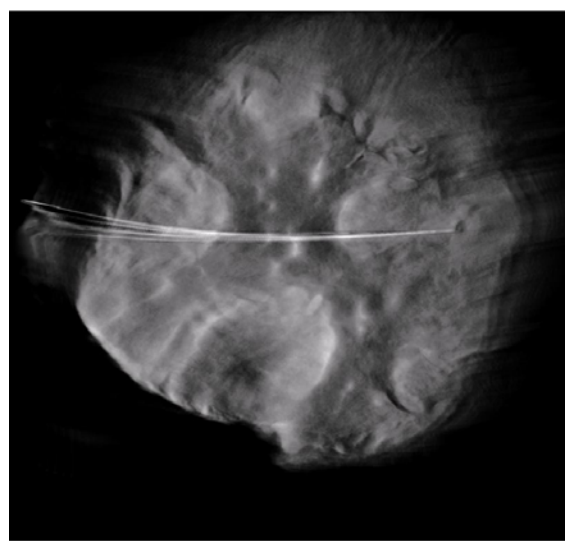
Tomosynthesis reconstruction of a 1 mm slice 40 mm from the surface of specimen.
